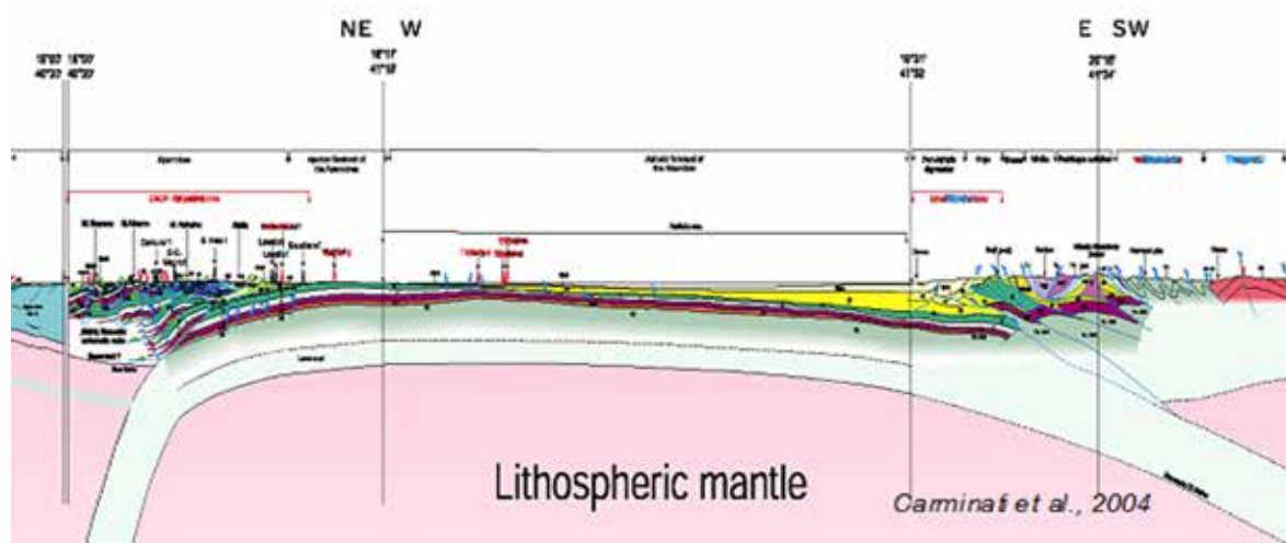
Figure 2 Relation between Apennines and Albanides
