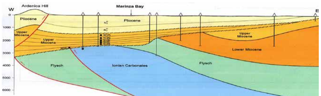
Fig. 11 Geological Cross Section – Mariza Oil Field Albania
