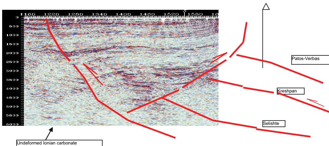
Figure 15 Onshore Seismic line (above Marinza oil field)
