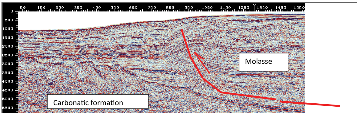
Figure 16 Offshore Seismic line
