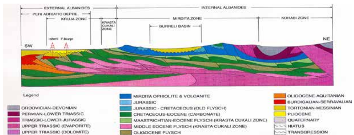
Fig. 6 Cross section I-I
