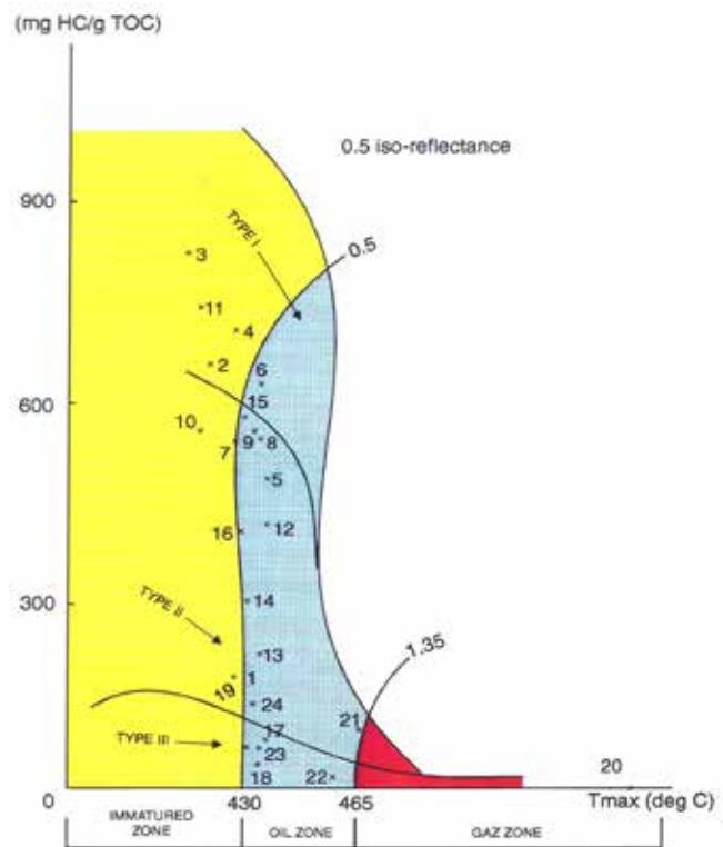
Fig. 8 Type and Maturity of Organic Mater
