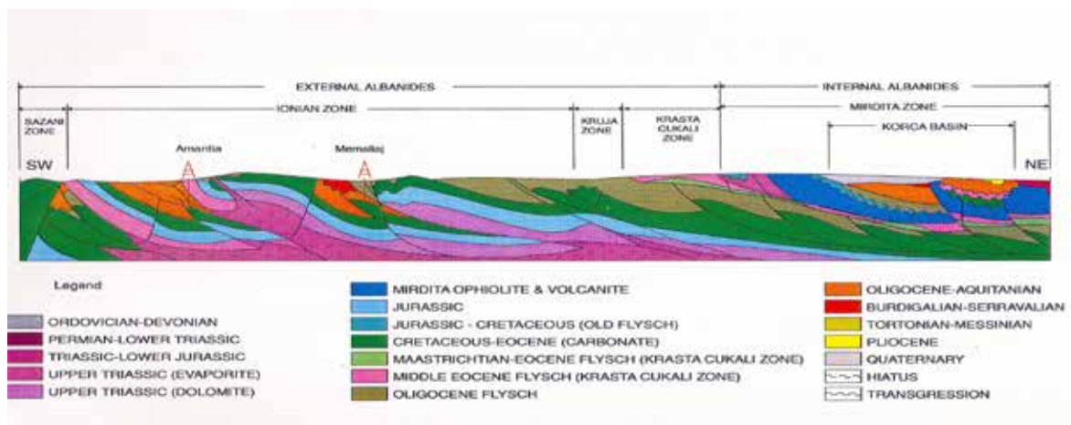
Fig. 7 Cross section II-II
