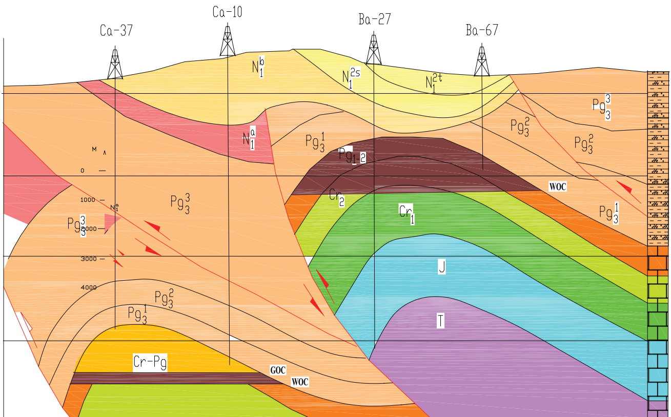
Fig. 10 Cakrani and Ballshi fields (limestones)
